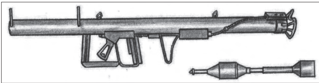
Rocket propelled grenade launcher, model 1943 (Raketenpanzerbüchse 43), caliber 88 mm, and its projectile, the R.P.G. 4322
