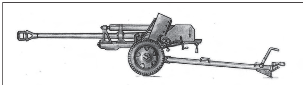
Antitank gun „D.T.-U.D.R.” no. 26, known under the name of „Reșița”, model 1943, caliber 75 mm
